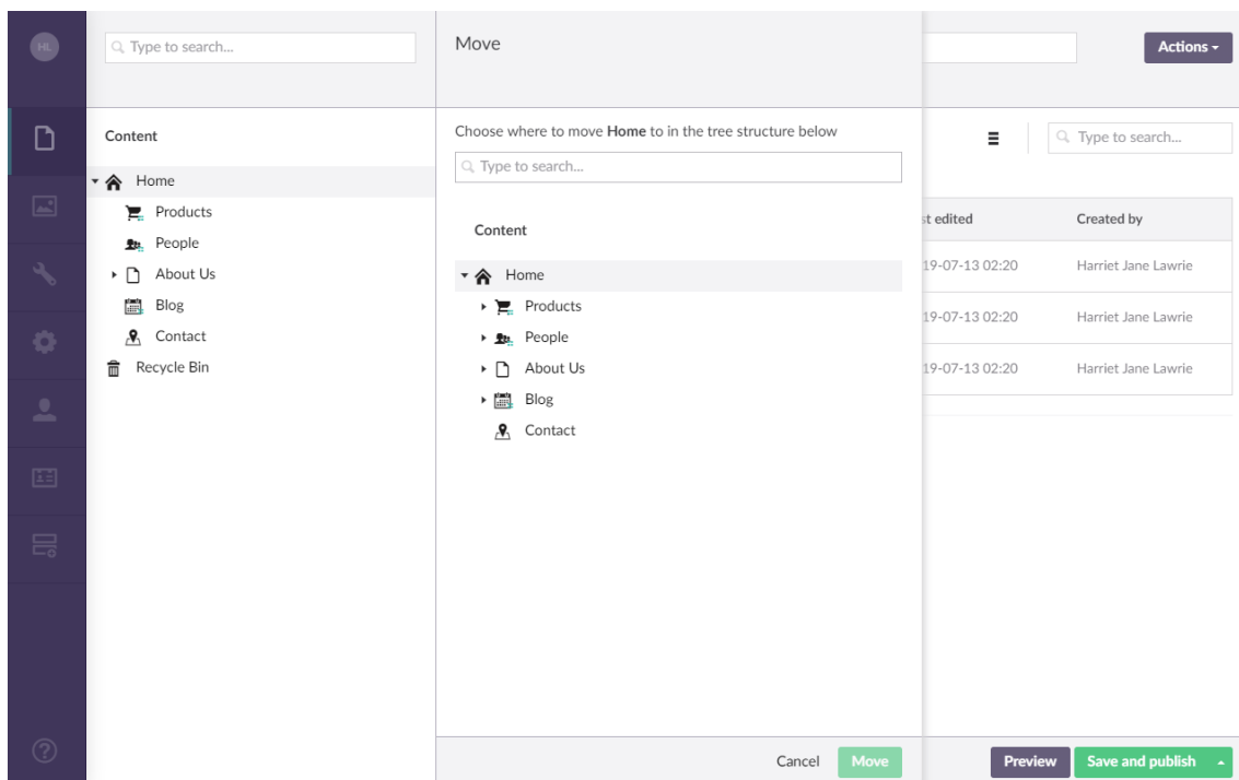
Screenshot 14 - Slide out menu for moving a page
